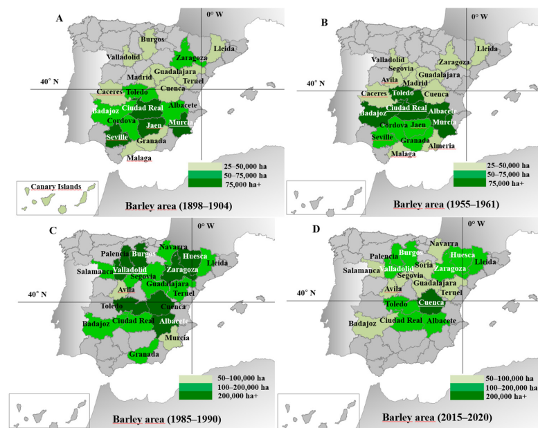
Figure 3. Provinces with the largest historical planted area of barley in Spain. Note the scale change for the area of (A,B) (smaller) with respect to (C,D). The five provinces with the largest planted area are white-lettered, and the main province is underlined [2].
